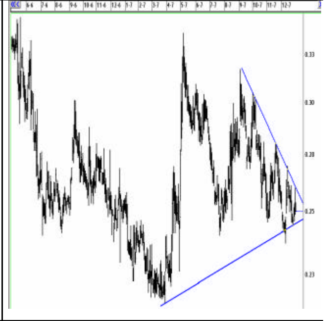
ALKA/IMKB (2006-2008)
